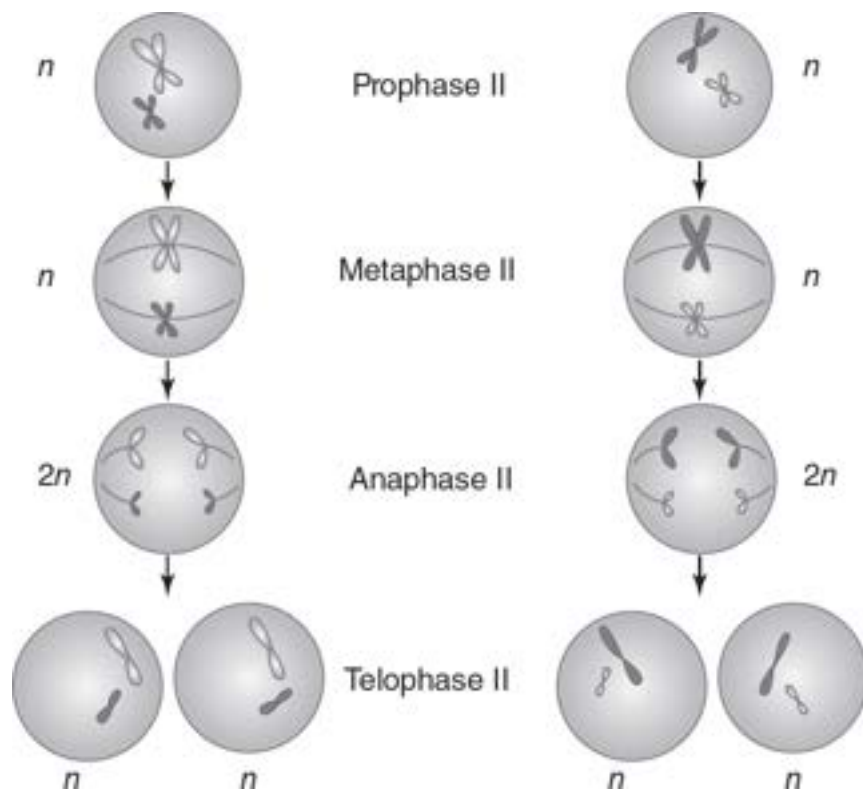
Figure 12.2 Meiosis II
