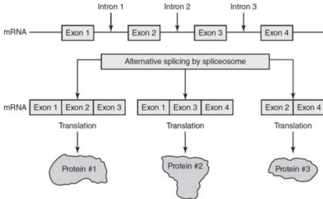
Figure 16.1 Alternative Splicing
