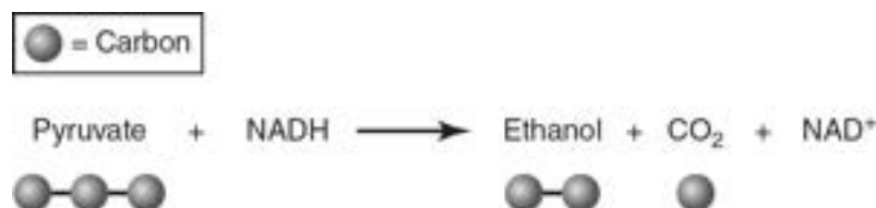
Figure 9.6 Alcohol Fermentation
