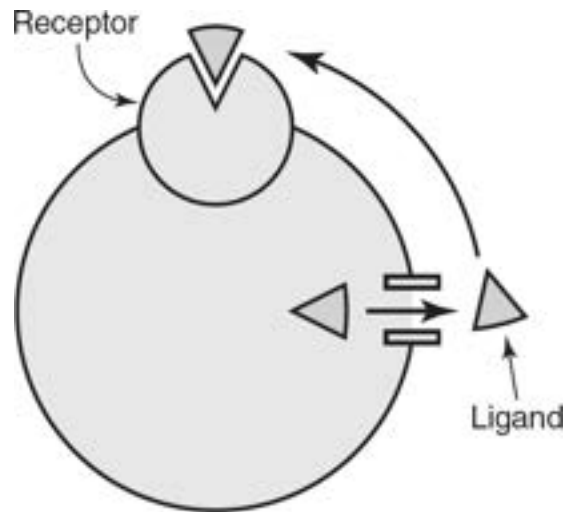
Figure 10.1 Autocrine Signaling
