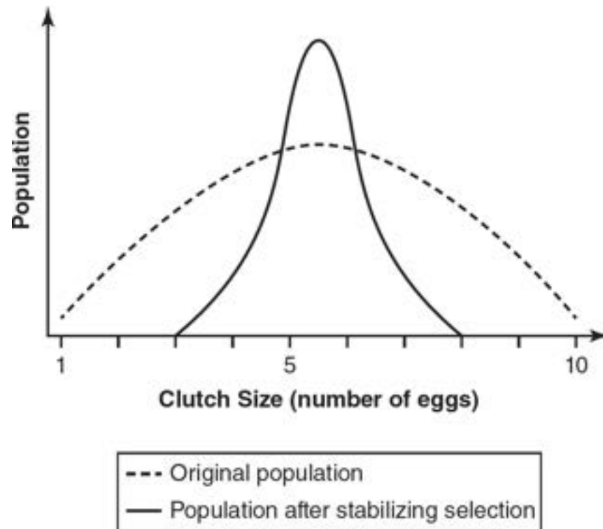
Figure 19.4 Stabilizing Selection
