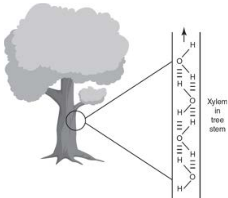
Figure 3.3 Capillary Action
