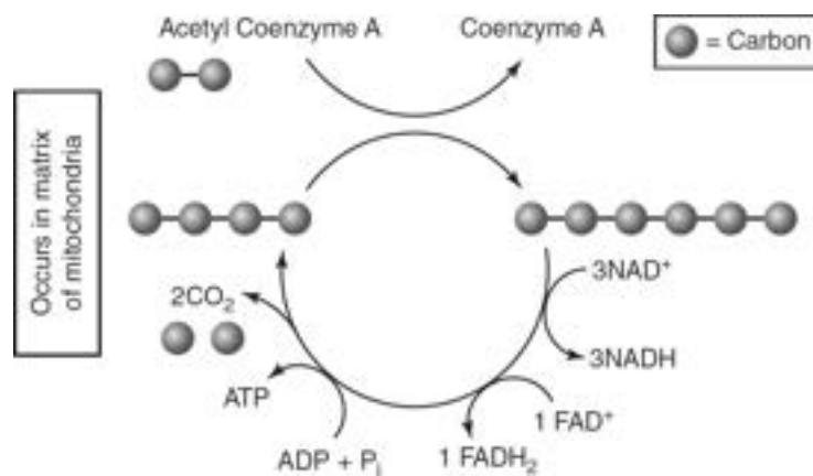
Figure 9.3 Krebs Cycle
