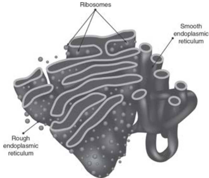
Figure 5.3 Endoplasmic Reticulum
