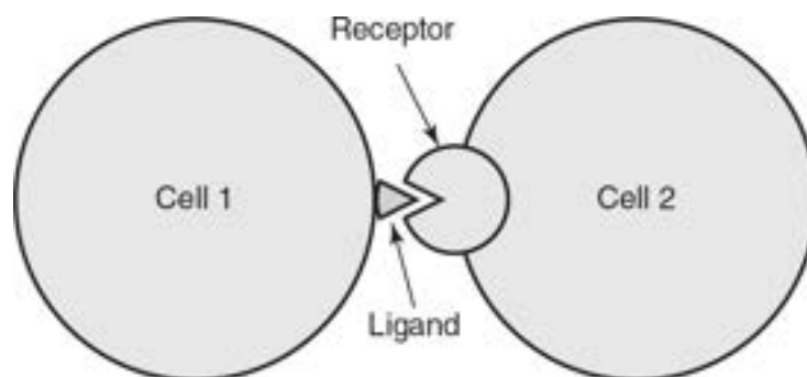
Figure 10.2 Juxtacrine Signaling
