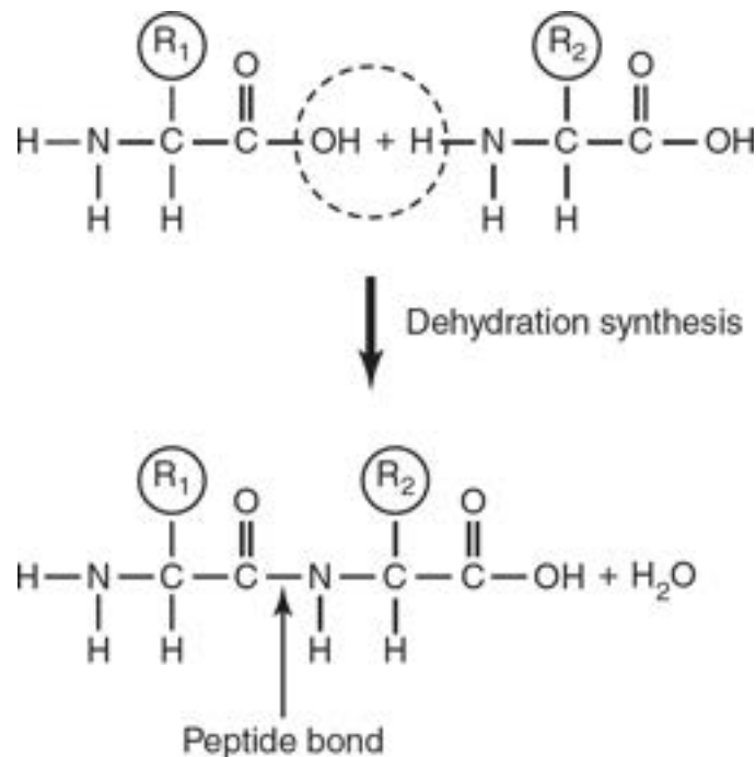
Figure 4.6 Peptide Bond
