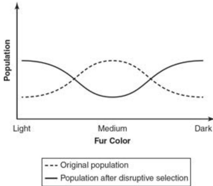
Figure 19.5 Disruptive Selection
